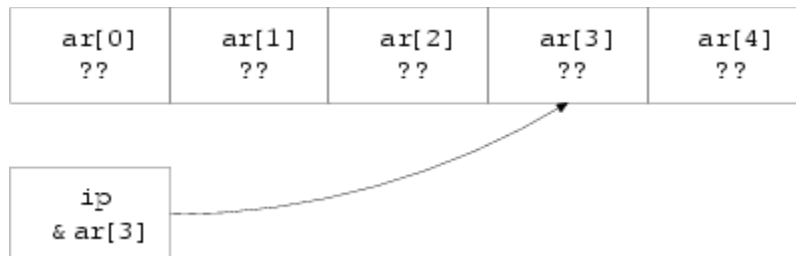
Figure 5.5 - Array and initialized pointer
