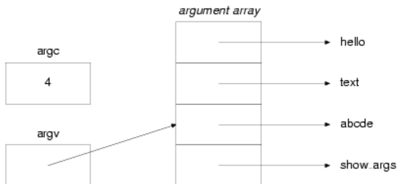
Figure 1.15 - Arguments to a program after incrementing argv
