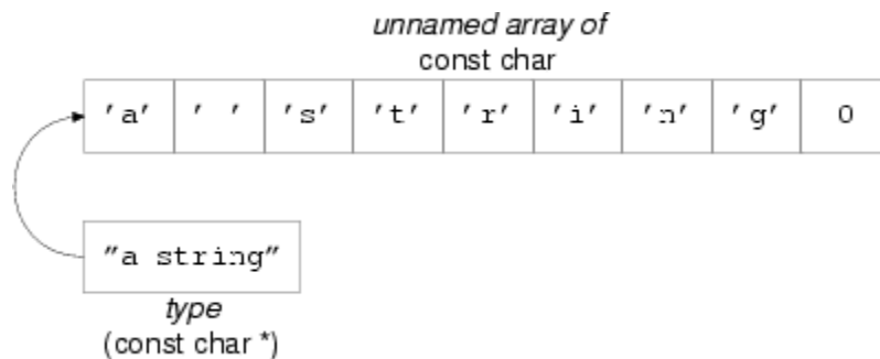
Figure 5.8 - Effect of using a string
