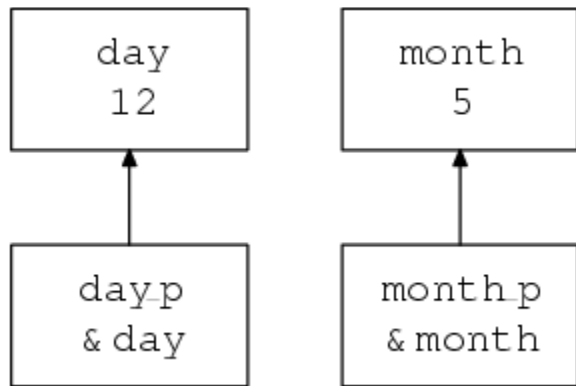
Figure 5.7 - Just as date is about to return
