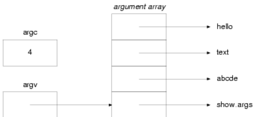
Figure 1.14 - Arguments to a program
