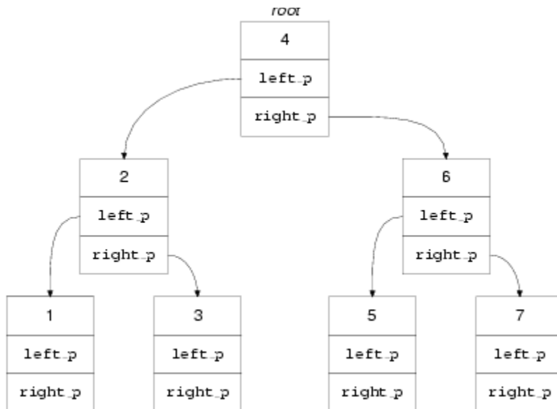
Figure 6.11 - A tree
